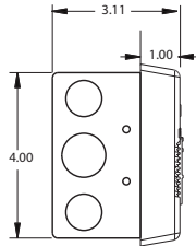
Flush Mount Side View
