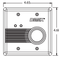
Flush Mount Front View
