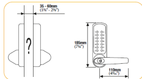
Model 600/605 For use with existing lock
