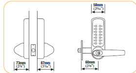
Model 610/615 With tubular latchbolt
