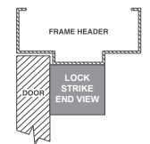
Surface Mount Outswing Door
